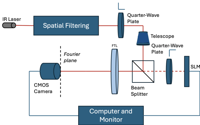
Figure 4: Optical setup for the joint transform correlator. The SLM displays the reference and query patterns side by side.
